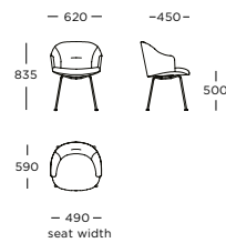
Chair V2 Tube base
